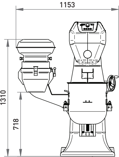
Machine with attachment device
