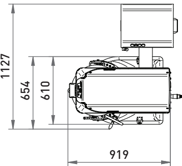
Machine without attachment device
