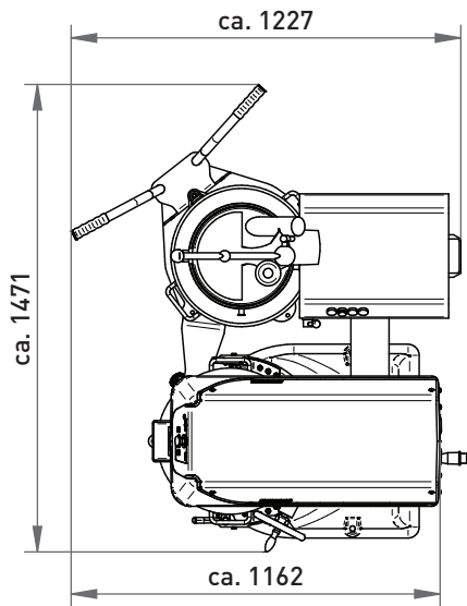
Machine with attachment device and trolley
